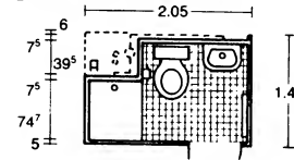
⑦ Shower cubicle with service duct
